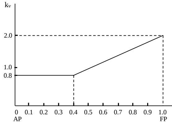
Fig. II 2-1 Acceleration Distribution k_v
