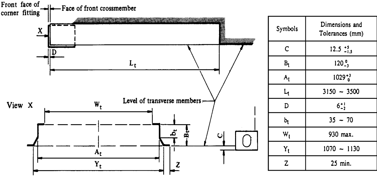
Fig. 5-3 Gooseneck Tunnel
