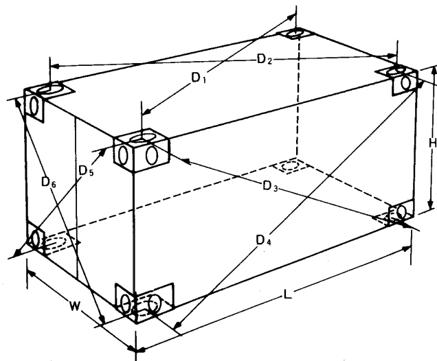
Fig. 3-1 Diagonal Tolerances
