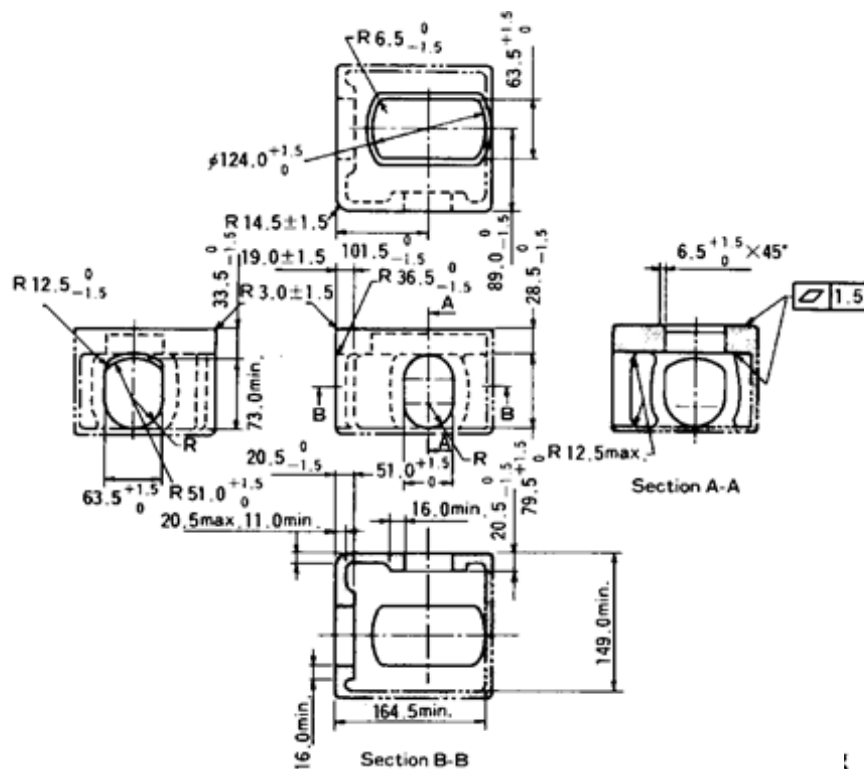
Fig. 3-2 Top Corner Fitting (Dimensions in mm)
